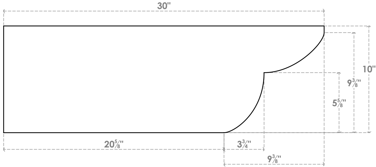
SIDE PROFILE
